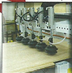
Automatic Load
